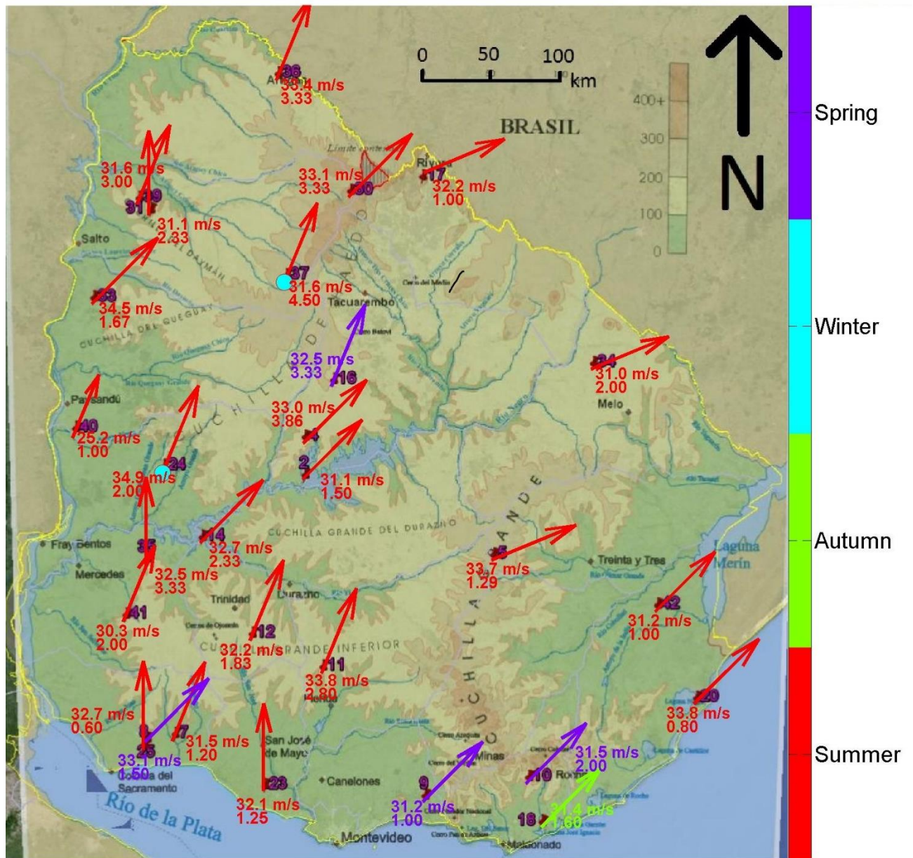
Figure 2. Location of stations and characteristics of the events with U_{\text{gust } 45\text{m}} \geq 29\text{m/s} .
